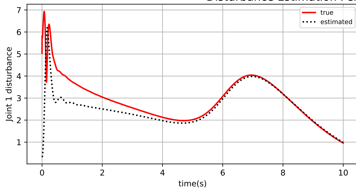
Disturbance Estimation Performance (S=3, S1=2, m=5)
